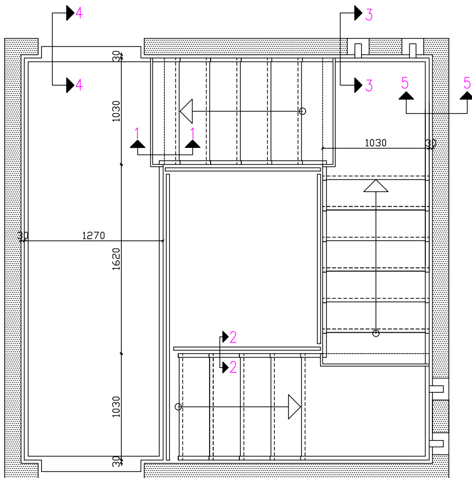
Plan of Trapperum
