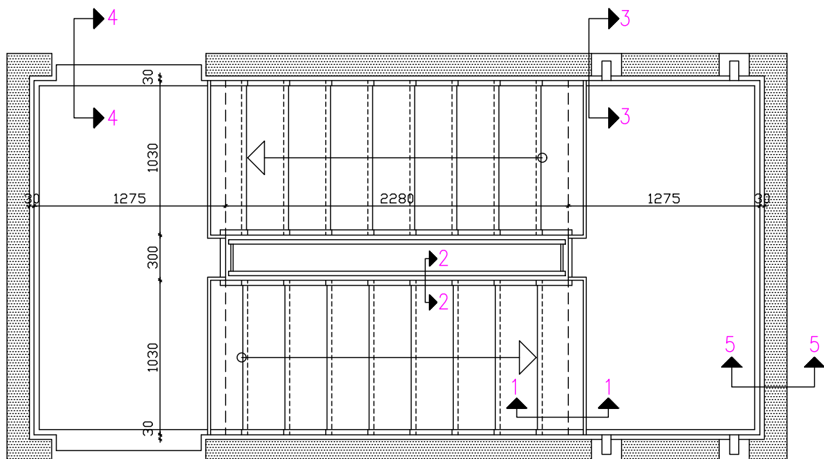
Plan of Trapperum
