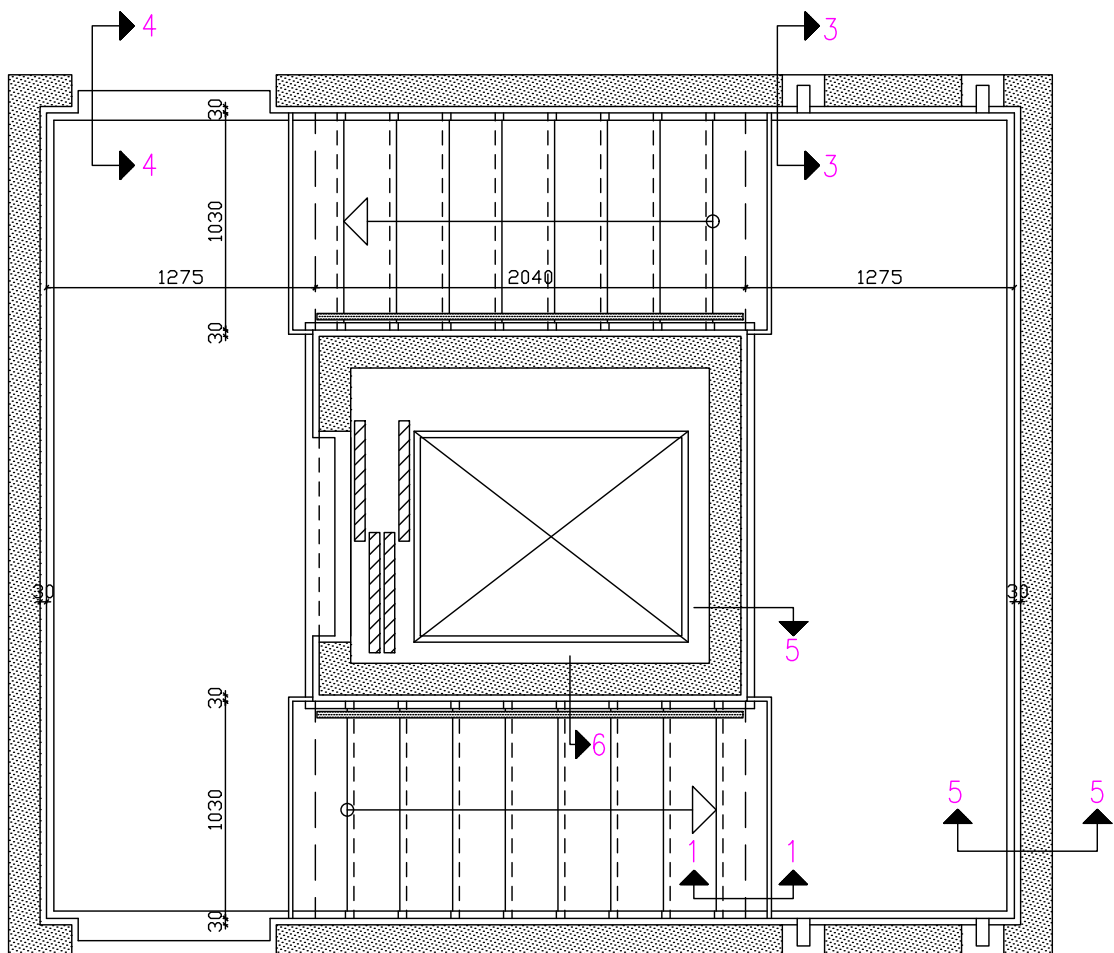
Plan of Trapperum
