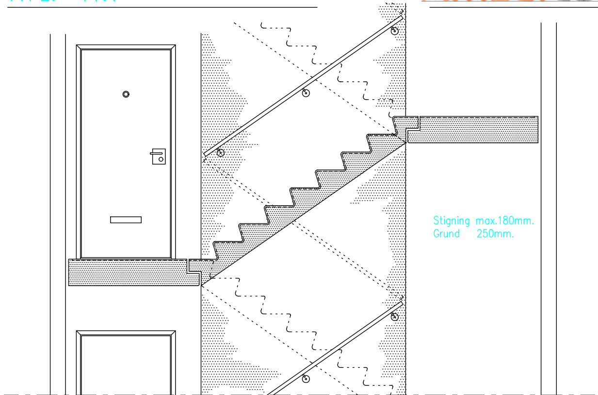
Opstalt of Trapperum
